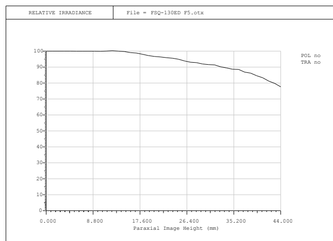
Relative Illumination
